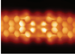
STM image of a graphene nanoribbon in which a seven-carbon-atom armchair configuration doped by a pair of boron atoms builds up a net magnetic moment. [N. Friedrich et al. , Phys. Rev. Lett. 125 , 146801 (2020)]
