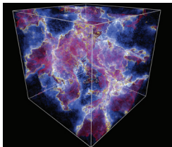
String network (yellow strings), domain walls (red mesh), and energy density of the axion field (blue-white intensity) during the QCD phase transition. [M. Buschmann, J. W. Foster, and B. R. Safdi, Phys. Rev. Lett. 124 , 161103 (2020)]
