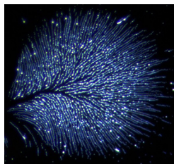
Microscopic image of a single droplet cluster at the interface between a nematic liquid crystal and air. [N. Wang et al. , Phys. Rev. Lett. 123 , 087801 (2019)]
