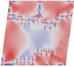
Collective dislocation nucleation pattern in a two-dimensional square lattice subjected to uniform shearing. Colors indicate the level of stress. [R. Baggio et al. , Phys. Rev. Lett. 123 , 205501 (2019)]
