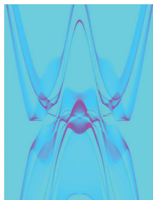
The gapped (001) surface states of transition metal dichalcogenide \beta -MoTe 2 calculated from first principles. [Zhijun Wang et al. , Phys. Rev. Lett. 123 , 186401 (2019)]
