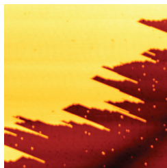
Large-scale STM image of a cleaved \text{Fe}_3\text{Sn}_2 surface with two different surface layers: Fe-Sn (yellow) and Sn (red). Selected for an Editors' Suggestion. [Z. Lin et al. , Phys. Rev. Lett. 121 , 096401 (2018)]
