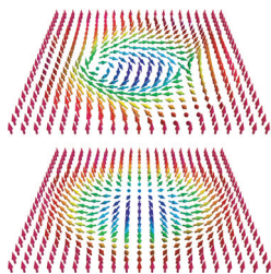
Schematic pictures of Bloch-type (top) and Néel-type (bottom) spin textures in Rashba metals. [S. Hayami and Y. Motome, Phys. Rev. Lett. 121 , 137202 (2018)]
