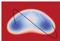
Double-well potential in two dimensions, plotted as a heat map. The wells are marked by green dashed circles and three examples of paths between them are shown (black, gray and white lines). [Peter G. Bolhuis and Gábor Csányi, Phys. Rev. Lett. 120 , 250601 (2018)]
