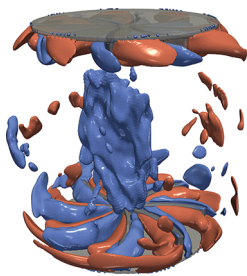
Magnetic field isocontours from an MHD simulation of a dynamo instability. [S. Kreuzahler et al. , Phys. Rev. Lett. 119 , 234501 (2017)]
