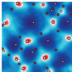
Lorentz micrograph of a network of clockwise and anticlockwise vortices (white) and achiral antivortices (red) in a thin iron film. [Tim Eggebrecht et al. , Phys. Rev. Lett. 118 , 097203 (2017)]
