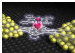
Molecular spin transistor with TbPc 2 molecule embedded between two gold tips. [F. Troiani et al. , Phys. Rev. Lett. 118 , 257701 (2017)]
