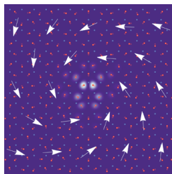
Waveguide lattice for the generation of photonic topological zero modes. [Thomas Iadecola, Thomas Schuster, and Claudio Chamon, Phys. Rev. Lett. 117 , 073901 (2016)]
