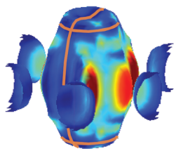
Calculated superconducting gap amplitude on one of the orbital-resolved Fermi surfaces of UPt 3 for a candidate pairing state. Three line nodes are highlighted in orange. [Takuya Nomoto and Hiroaki Ikeda, Phys. Rev. Lett. 117 , 217002 (2016)]
