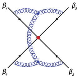
A three-loop connected web contributing to the soft anomalous dimension governing long-distance singularities of multileg gauge-theory scattering amplitudes of massless partons. [Øyvind Almeliid, Claude Duhr, and Einan Gardi, Phys. Rev. Lett. 117 , 172002 (2016)]
