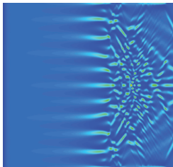
Simulated propagation in the x - z plane of perturbed extended modes of a cavity-free laser with a graphene-based active random metamaterial as amplifying medium. [A. Marini and F. J. García de Abajo, Phys. Rev. Lett. 116 , 217401 (2016)]
