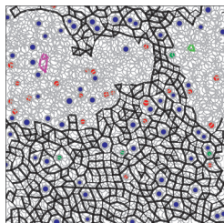
Simulated frictional packings of polydisperse disks decompose into rigid clusters (black, purple, and green) and regions of floppy bonds (gray). [Silke Henkes et al. , Phys. Rev. Lett. 116 , 028301 (2016)]
