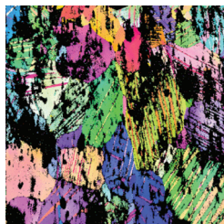
Electron backscattered diffraction scan of a deformed Re-W alloy with abundant twinning. Black areas represent surface pitting. [Maarten de Jong et al. , Phys. Rev. Lett. 115 , 065501 (2015)]
