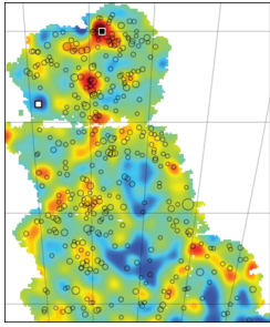
Weak gravitational lensing map for 139 \text{ deg}^2 of the sky from the Dark Energy Survey. Overdense regions (red) are in good agreement with the locations of galaxy clusters (circles). Selected for an Editors' Suggestion and a Viewpoint in Physics . [C. Chang et al. , Phys. Rev. Lett. 115 , 051301 (2015)]
