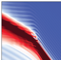
Graph showing longitudinal resistance at finite magnetic field as a function of top and bottom gate voltages for an InAs/GaSb double quantum well device. [Fanming Qu et al. , Phys. Rev. Lett. 115 , 036803 (2015)]
