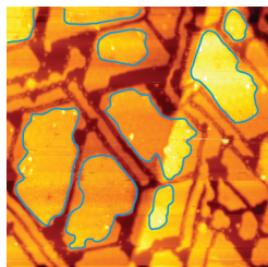
STM topograph of Eu-intercalated graphene (bright) and nonintercalated graphene (dark) on Ir(111) with naphthalene islands (outlined in blue) atop Eu-intercalated patches. Selected for an Editors' Suggestion and a Synopsis in Physics . [F. Huttmann et al. , Phys. Rev. Lett. 115 , 236101 (2015)]
