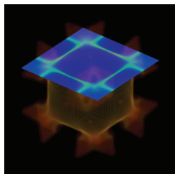
Three-dimensional Fermi surface of paramagnetic GdMg. A constant- k_z slice through the Fermi surface is highlighted in blue. [L. Petit et al. , Phys. Rev. Lett. 115 , 207201 (2015)]
