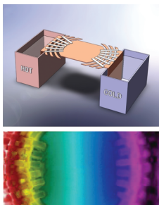
Design for demonstration of a macroscopic thermal diode, conducting case; heat is conducted from left to right (top). Experimentally measured temperature distribution of the device (bottom). [Ying Li et al. , Phys. Rev. Lett. 115 , 195503 (2015)]
