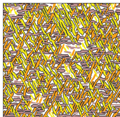
Amyloid fibril network simulation for 31130 peptides on a 2D lattice. [L. G. Rizzi, D. A. Head, and S. Auer, Phys. Rev. Lett. 114, 078102 (2015)]
