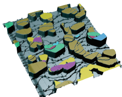
Scanning tunneling microscope image of the topography of Pb islands on a Cu(111) surface. [M. Shackert et al. , Phys. Rev. Lett. 114 , 047002 (2015)]
