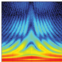
Number of x-ray photons (color) as a function of time (vertical) and detuning (horizontal) shows that near-resonant pulses are delayed. Selected for an Editors' Suggestion and a Viewpoint in Physics . [K. Heeg et al. , Phys. Rev. Lett. 114 , 203601 (2015)]
