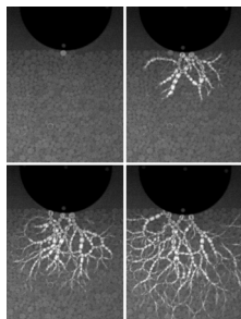
High-speed video images showing force propagation through a granular material made of photoelastic particles after impact by a large bronze disk. [Abram H. Clark et al. , Phys. Rev. Lett. 114 , 144502 (2015)]
