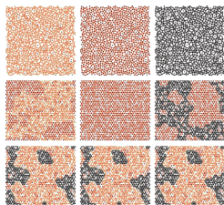
Pebble game analysis of network topologies for a jammed packing (top), stress-relieved triangular network (middle), and rigidity percolation (bottom). [Wouter G. Ellenbroek et al. , Phys. Rev. Lett. 114 , 135501 (2015)]
