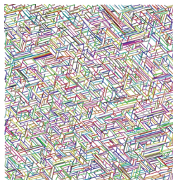
Model network obtained from a feature extraction program applied to an AFM scan of a triaxial collagen network. Filaments are individually recognized and colored randomly. [Wonmuk Hwang and Esma Eryilmaz, Phys. Rev. Lett. 113 , 025502 (2014)]
