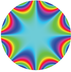
Calculated reciprocal space wave function of an electron probe beam distorted by fourfold astigmatism. [J. Ruzs, J.-C. Idrobo, and S. Bhowmick, Phys. Rev. Lett. 113 , 145501 (2014)]
