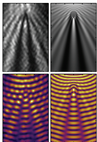
Experimental (left) and simulated (right) real-space optical intensity and interference patterns of a linear polariton wave in a GaAs microcavity propagating across a pointlike defect. [P. Cilibrizzi et al. , Phys. Rev. Lett. 113 , 103901 (2014)]
