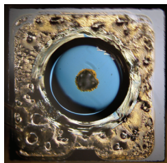
Avalanche photodiode damaged by a high power laser beam during a cryptography attack. The dark central spot is a hole blown through the chip. Selected for a Synopsis in Physics . [A. Bugge et al. , Phys. Rev. Lett. 112 , 070503 (2014)]
