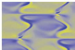
Simulation of Taylor-Couette fluid flow. Blue (yellow) represents positive (negative) azimuthal vorticity. [K. Deguchi, A. Meseguer, and F. Mellibovsky, Phys. Rev. Lett. 112 , 184502 (2014)]
