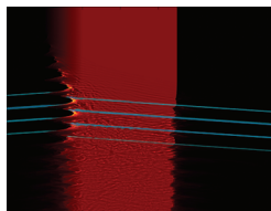
Simulation of attosecond pulse generation (cyan) with electron density plotted against time (vertical) and position (horizontal) during a laser-plasma interaction. [M. Yeung et al. , Phys. Rev. Lett. 112 , 123902 (2014)]
