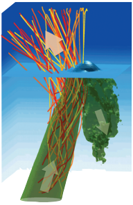
Electron deflection in a 3D simulation of laser-plasma interaction. Incident and reflected laser envelopes shown as green isosurfaces, fast electron trajectories in orange, and plasma density in blue, the slice showing the critical electron density. [F. Pérez et al. , Phys. Rev. Lett. 111 , 245001 (2013)]
