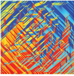
Simulated domain structure of a 1000 nm \times 1000 nm ferroelectric nanodot. Colors indicate the domain orientation: red, up; blue, down; cyan, left; yellow, right. [R. Ahluwalia, N. Ng, A. Schilling, R. G. P. McQuaid, D. M. Evans, J. M. Gregg, D. J. Srolovitz, and J. F. Scott, Phys. Rev. Lett. 111 , 165702 (2013)]
