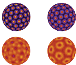
Density profiles for composite fermion crystals on the surface of a sphere. [Alexander C. Archer, Kwon Park, and Jainendra K. Jain, Phys. Rev. Lett. 111 , 146804 (2013)]
