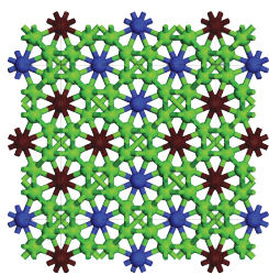
Crystalline structure of the Ca-VII superconducting phase of calcium. [H. Fujihisa et al. , Phys. Rev. Lett. 110 , 235501 (2013)]
