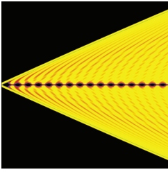
Scalar field as a function of space and time for a fixed Gaussian density distribution. For clarity, the unperturbed regions are shown in black. [Claudio Llinares and David F. Mota, Phys. Rev. Lett. 110 , 161101 (2013)]
