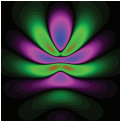
Snapshot of the Laplacian of the projected instantaneous electron density of a wave packet proposed to be imaged by scattering of ultrashort x-ray pulses. [Gopal Dixit, Jan Malte Slowik and Robin Santra, Phys. Rev. Lett. 110 , 137403 (2013)]
