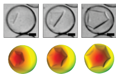
Optical microscope images of a colloidal capsule with an inhomogeneous shell, buckled under an external osmotic pressure; scale bar is 35 \mu\text{m} (top). Numerically simulated shell similar to the experimental capsule; color reflects spatially varying shell thickness (bottom). Elapsed time increases from left to right. [Sujit S. Datta et al. , Phys. Rev. Lett. 109 , 134302 (2012)]
