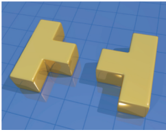
An artistic three-dimensional view of an example bow-tie nanoantenna consisting of eight gold cubes. [Thorsten Feichtner, Oleg Selig, Markus Kiunke, and Bert Hecht, Phys. Rev. Lett. 109 , 127701 (2012)]
