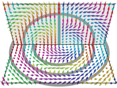
Pseudospin texture along the radial direction of a stable 3D skyrmion. [T. Kawakami et al. , Phys. Rev. Lett. 109 , 015301 (2012)]
