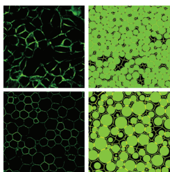
Tilings and tessellations of epithelial cells, bidisperse disks, compressed droplets and undeformed droplets. [K. A. Newhall et al. , Phys. Rev. Lett. 108 , 268001 (2012)]
