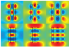
Calculated electric field distributions of two transverse electric modes (top and bottom) from three rectangular dielectric nanostrips with three different interstrip spacings (10, 31, and 80 nm). The red color indicates the highest field values, and blue the lowest. See article 053902.
