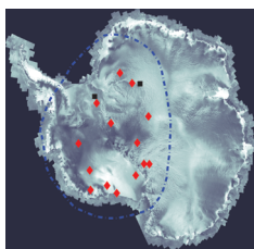
Locations of direct (black) and reflected (red) detection of ultrahigh energy cosmic ray events by the ANITA balloon experiment over Antarctica. The field of view is delineated by the dashed blue line. See article 151101
