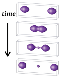
Zeptosecond snapshots of two ^{238}\text{U} nuclei colliding at 900 MeV, resulting in three primary fragments. See article 042701.
