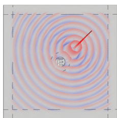
Flexural waves on a thin elastic plate are smoothly bent around an obstacle ("E") surrounded by a metamaterial cloak. See article 024301.
