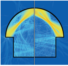
Spatial intensity of modes along marginally unstable periodic orbits in a mushroom-shaped cavity. Modes for two different values of wavelength and the ratio of frequency to energy decay rate are shown left and right. See article 154101.
