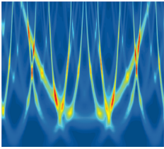
Time-energy plot of the expected event rate for finding photon-converted solar axions with a germanium detector. See article 141802.
