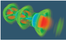
Wakefield created in a plasma illuminated by a laser, which results in emission of electro-optic shock radiation from the electron sheath (blue) around a plasma bubble (red). See article 045004.
